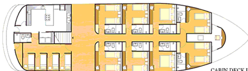
CABIN DECK I
